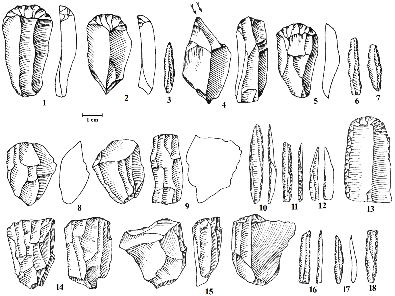
Figure 20: Warwasi artifacts P-U.1, 2, 5, 13) end scrapers; 3, 6, 7, 10, 12, 17, 18) different retouched bladelets, 11, 16) backed bladelets, 4, 8, 9, 14, 15) bladelet core (modified after Otte and Kozłowski 2007).
