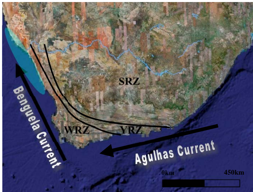
Figure 2.1 Map of South Africa showing the rainfall zones and dominant currents. Note the edge of the continental plateau. SRZ is summer rainfall zone, WRZ is winter rainfall zone, YRZ is year-round rainfall zone. The blue zone on the west coast shows the region of cold water upwelling. Image taken from Google Earth
