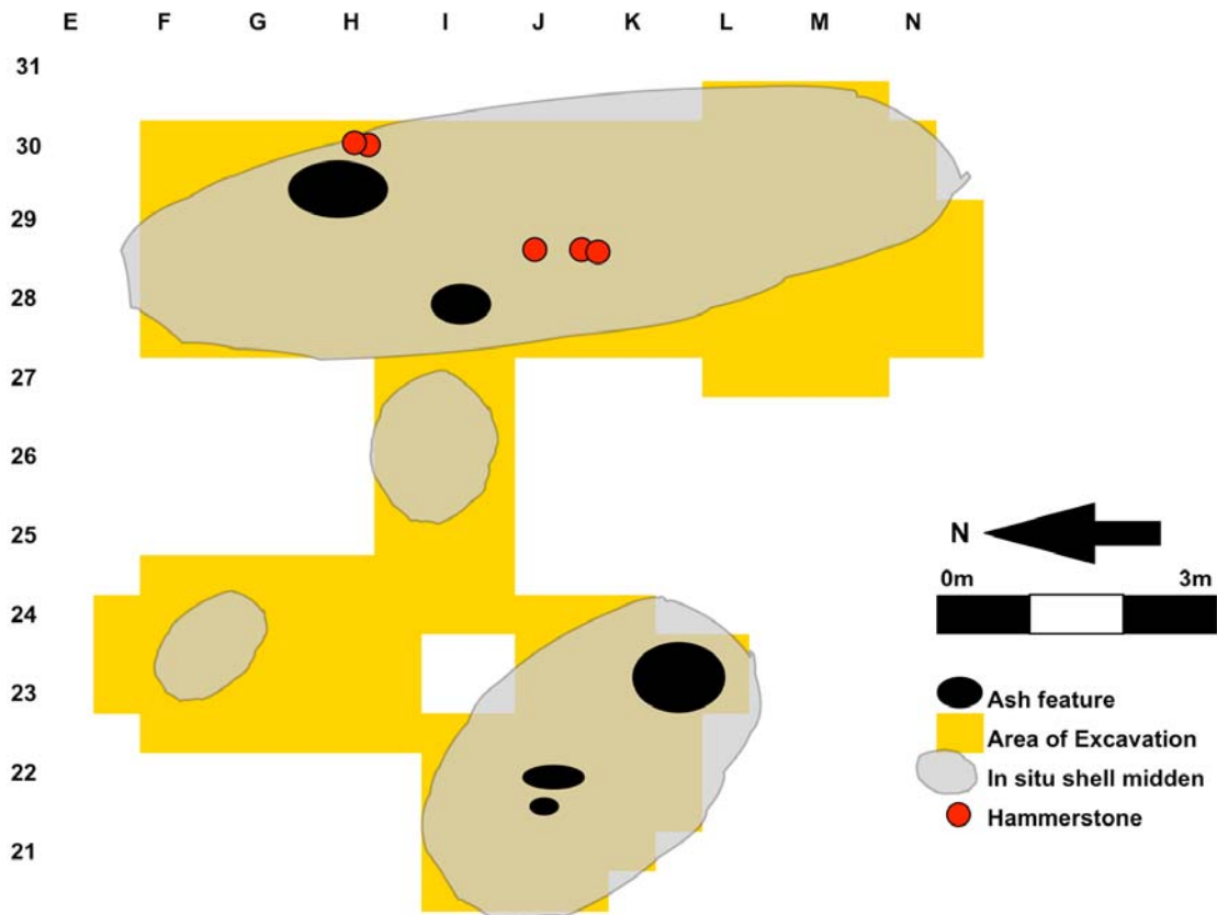
Figure 5.2 Plan of SK400
